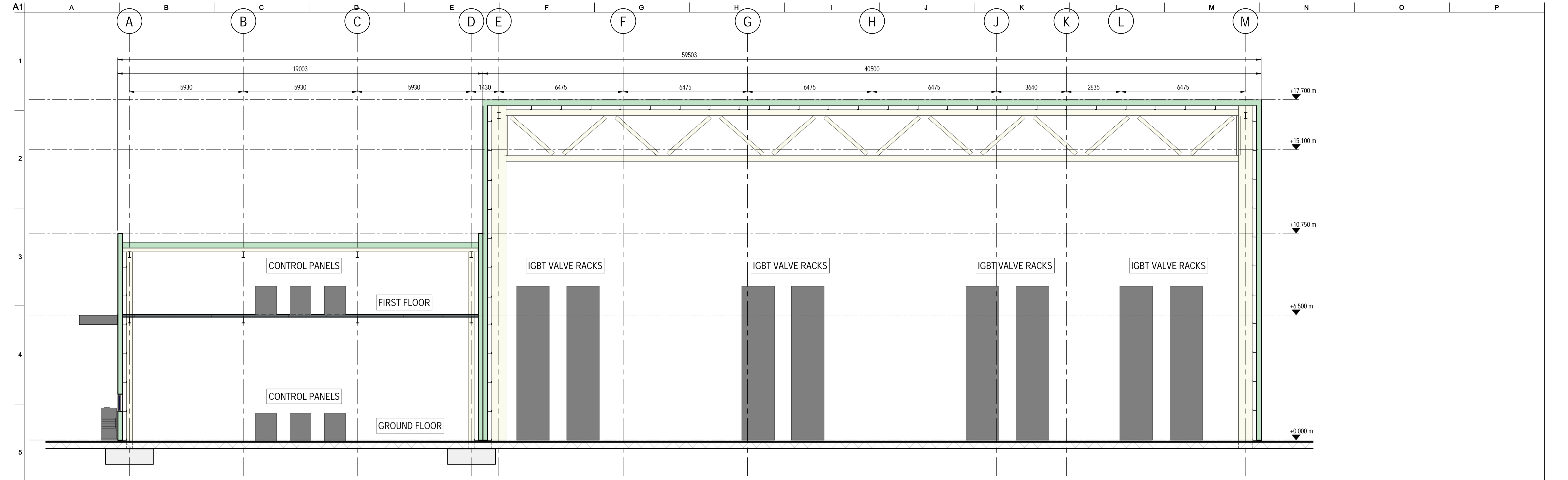
SECTION C-C SCALE 1:100
