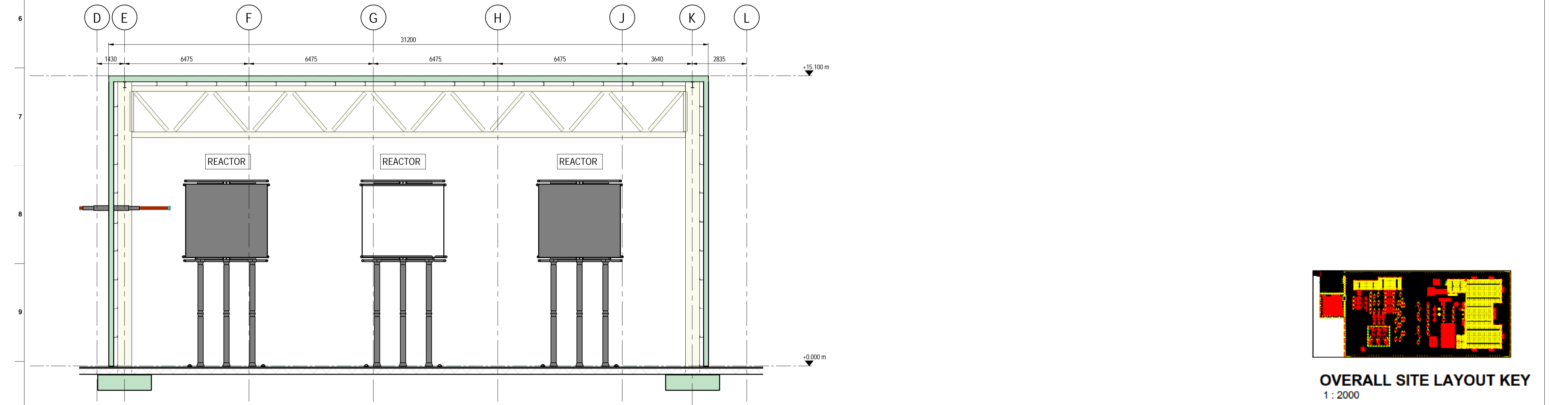
SECTION D-D SCALE 1:100
